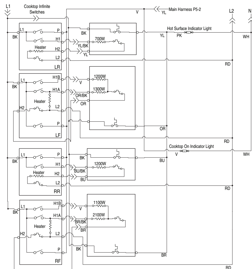
Cooktop Wiring Diagram
